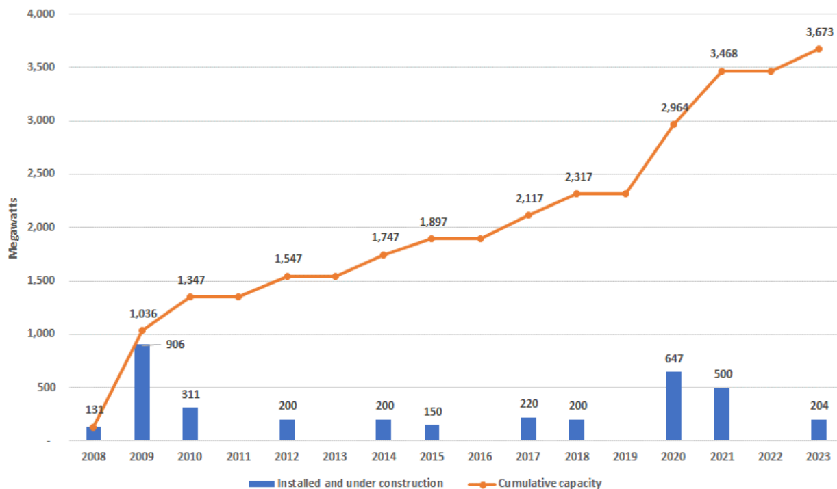
Figure 2-12: Utility-scale wind farm capacity installed and under construction in Indiana (Data source: DOE [11], IURC [25], EDP [26]).
