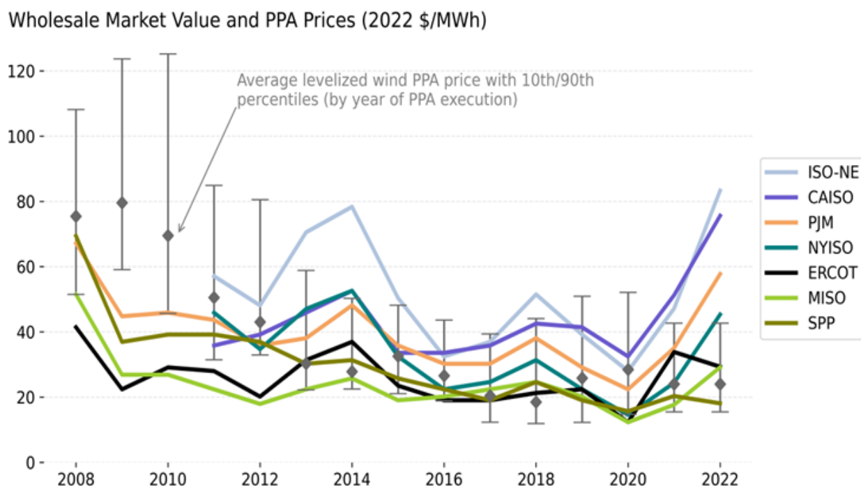
Figure 2-7: Wholesale energy value of wind (Source: LBNL [10])
