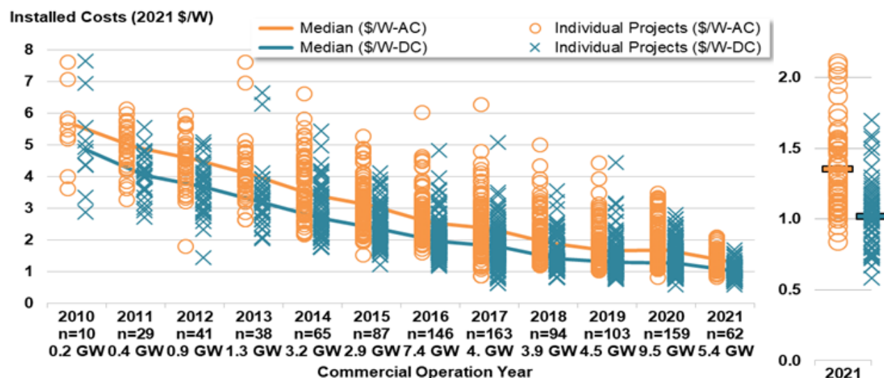
Figure 6-5: Installed cost of utility-scale PV systems over time (Source: LBNL [11])
