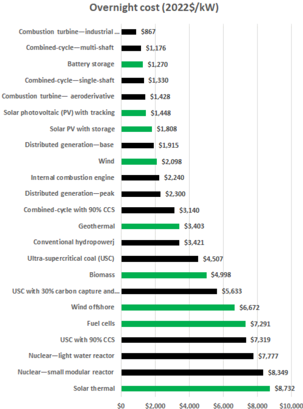
Figure 1-11: Estimated generating technologies capital costs (Data source: EIA [17])
