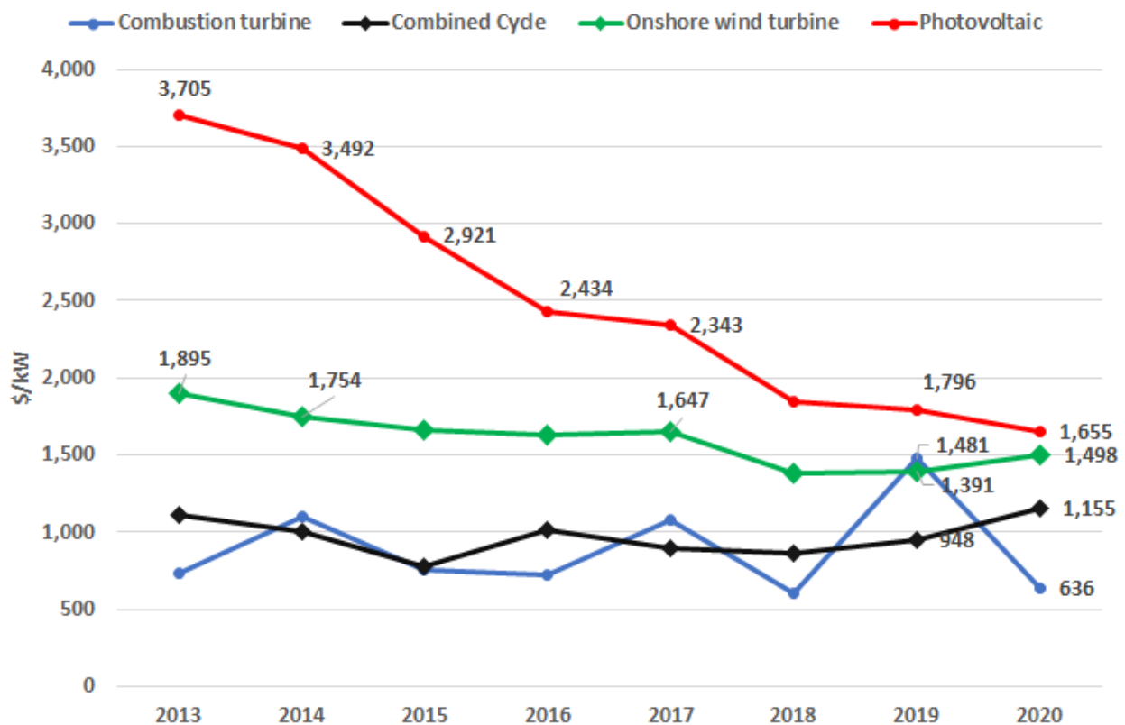
Figure 2-3: Average construction cost of generators installed 2013 to 2020 in the U.S. (Data source: EIA [8, 9])
