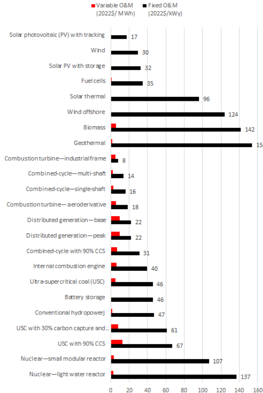
Figure 6-8: Estimated generating technologies fixed and variable O&M costs (Data source: EIA [13])
