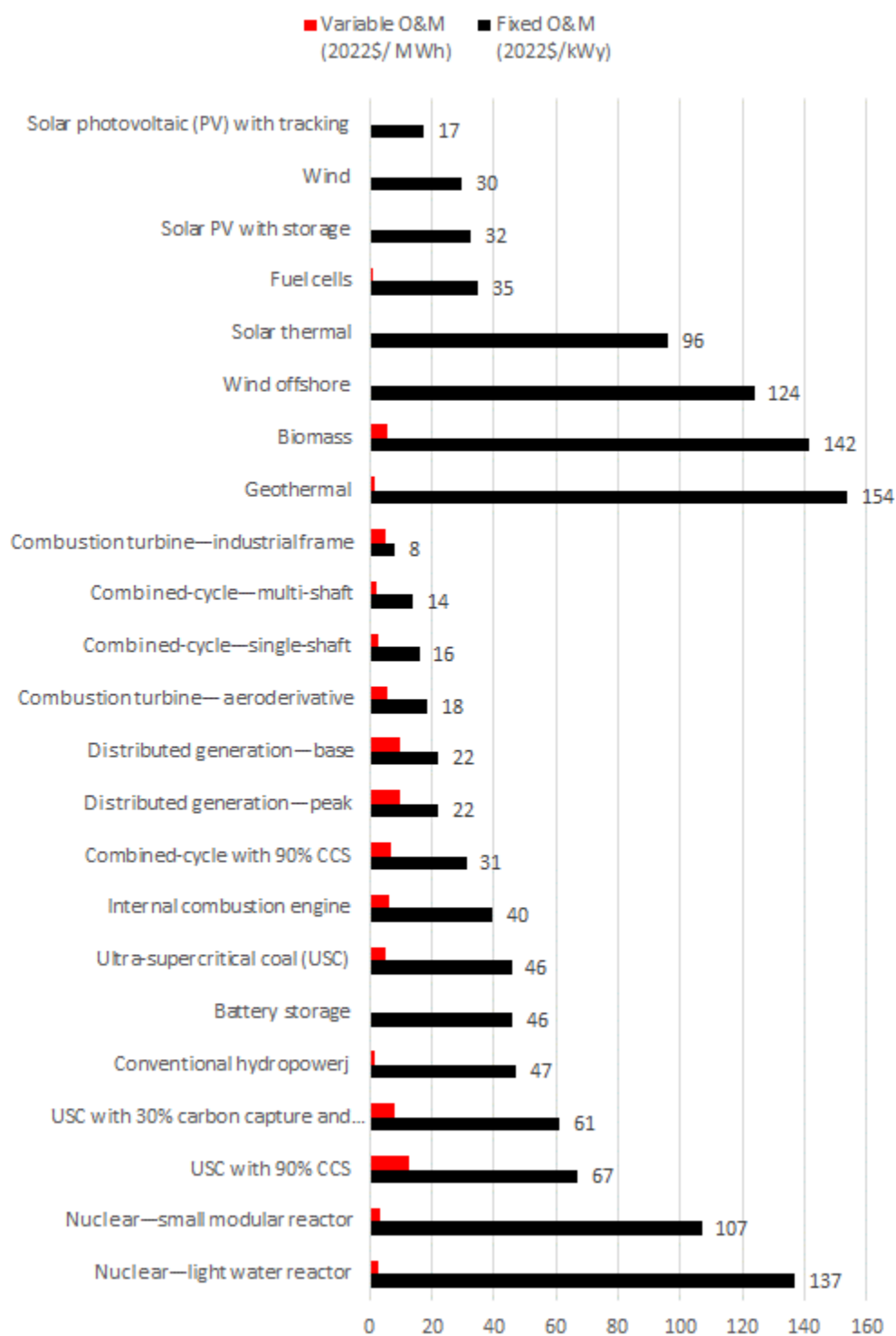
Figure 1-12: Estimated generating technologies fixed and variable O&M costs (Data source: EIA [17])
