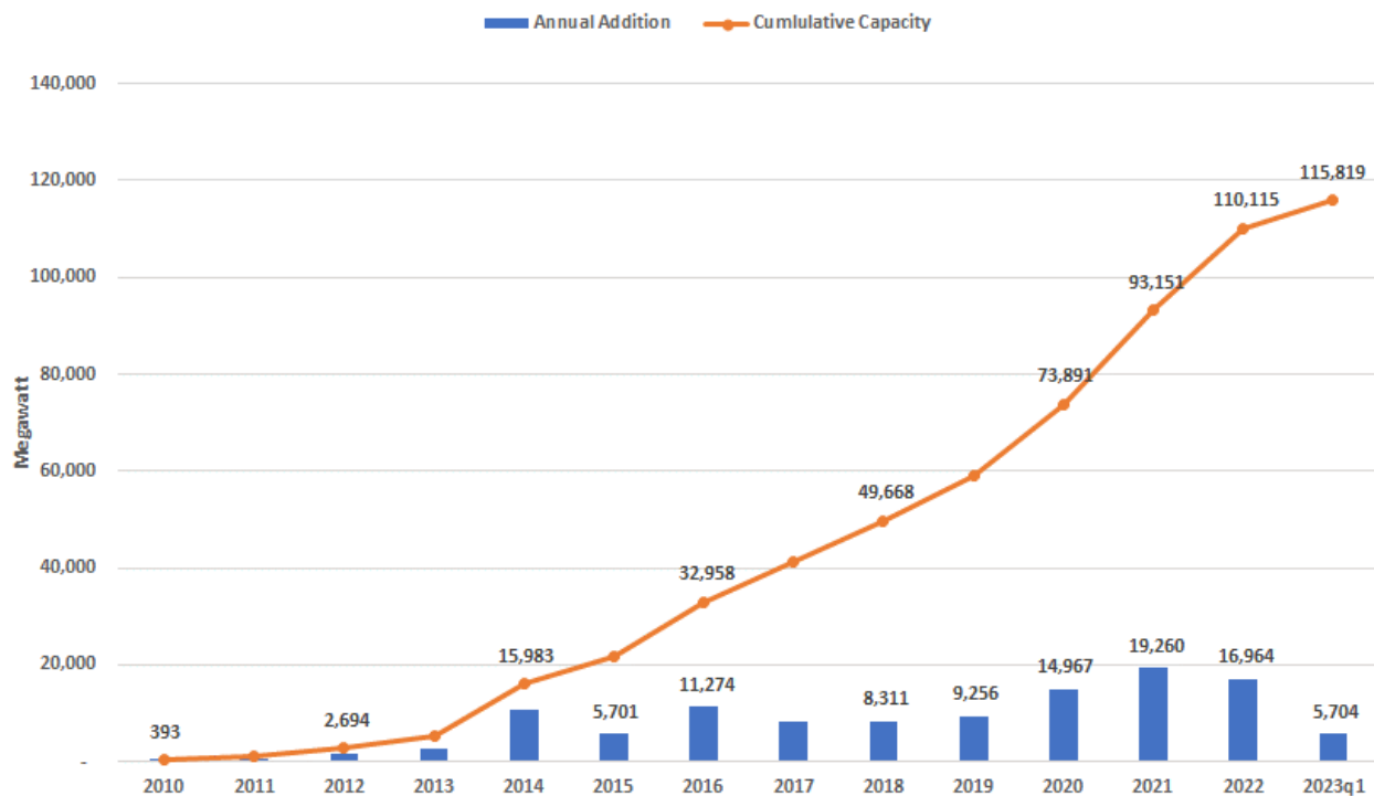
Figure 6-9: Installed U.S. PV capacity (Data source: EIA [4, 14])
