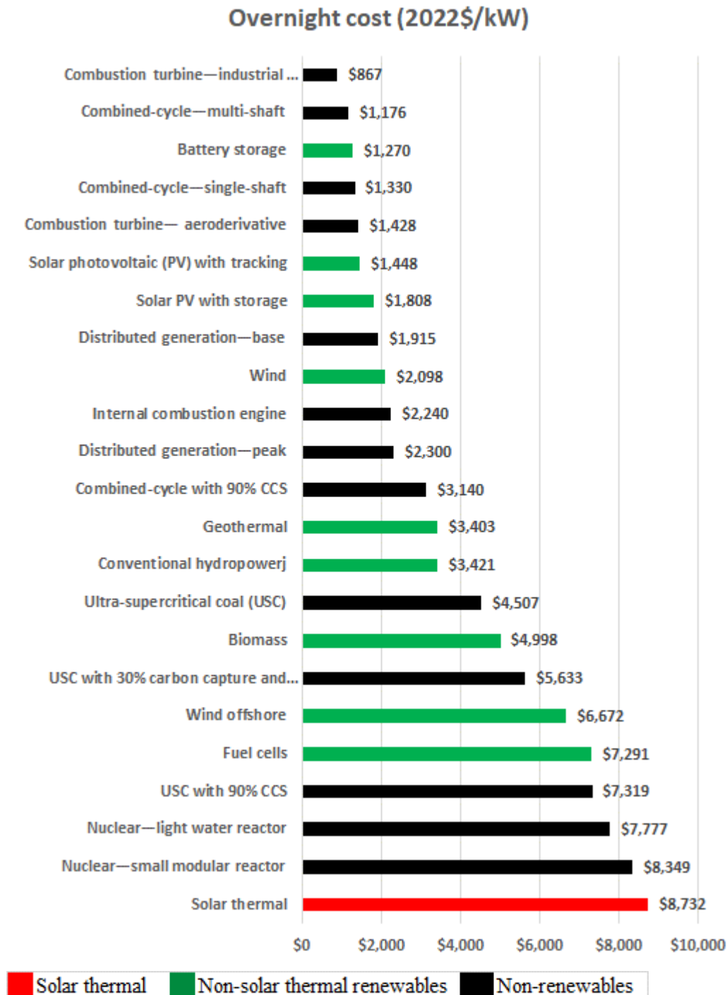
Figure 5-6: Estimated capital cost of generating technologies (Data source: EIA [5])
