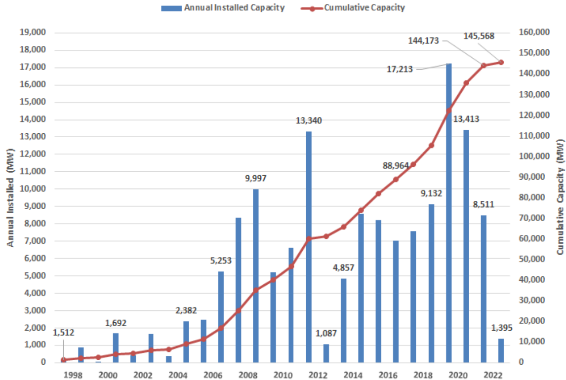
Figure 2-8: U.S. wind capacity growth (Sources: LBNL [10], DOE [11])
