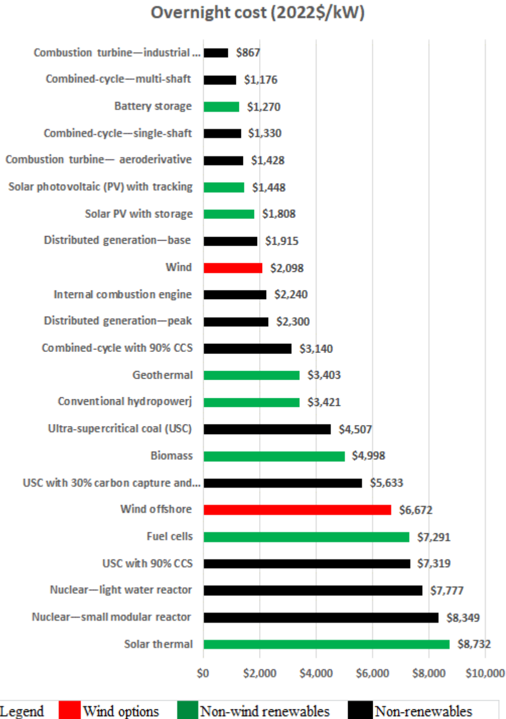
Figure 2-2: Estimated capital costs of various electric generation options (Data source: EIA [7])
