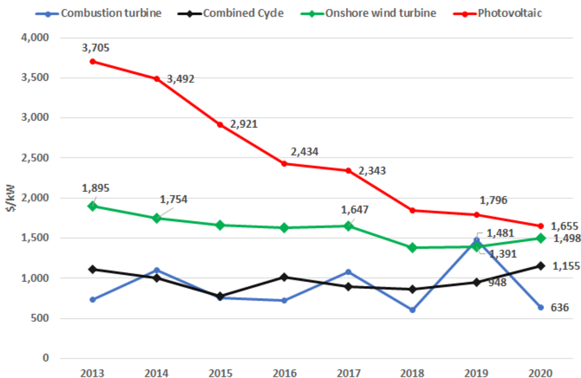
Figure 1-10: Average construction cost of generation installed 2013 to 2020 (Data source: EIA [16])
