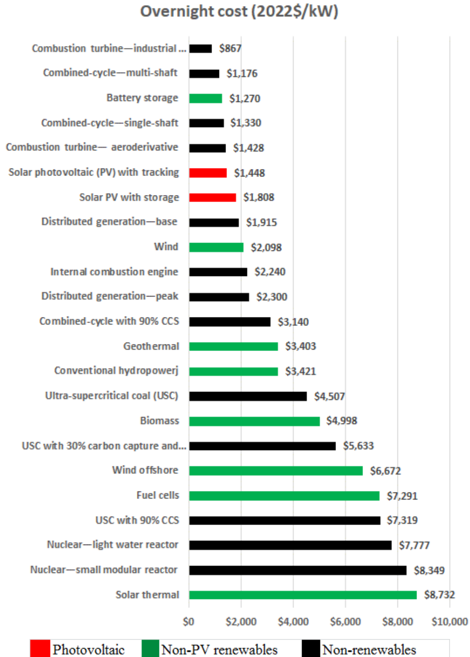
Figure 6-7: Estimated generating technologies capital costs (Data source: EIA [13])
